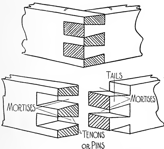
FIG. 267. DOVETAIL JOINT.
